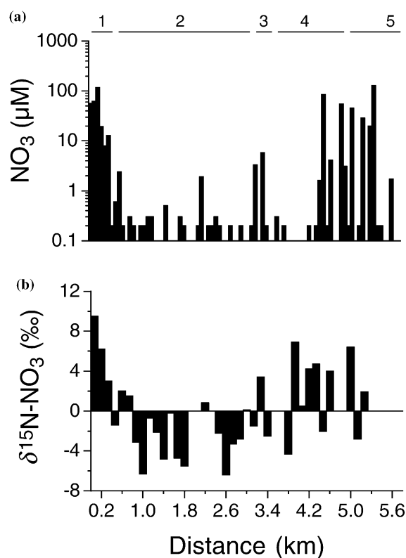
Figure 2. Example of variation of NO 3 concentrations (a) and isotope values (b) in seepage face water of an estuary of this study, Mashpee River. Concentrations for each 200 m composite were averaged across all seasons collected (summer, fall, winter). Numbered horizontal lines across top represent recharge zones delineated in Figure 1, and each line covers samples collected within that recharge zone. Distance along the x-axis is measured in a counter clock-wise direction from the eastern side of the river mouth to the western side of the river mouth. Stream water samples collected upstream of the tidal range represent Recharge Zone 3.
